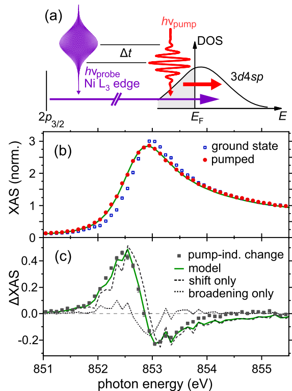
Figure 1. (a) Near-infrared pump, soft x-ray absorption probe experiment at the Ni L_3 absorption 2p_{3/2} \rightarrow 3d4sp analyzing the transiently modified electronic density of states above E_F at time delay \Delta t . (b) Ground state (blue squares) and pumped (circles) absorption spectrum at \Delta t = 0.4 ps. The pump-induced changes \Delta\text{XAS} are modeled (green line) based on the static absorption spectrum which allows to distinguish the contributions of an energy shift and broadening. (c) Pump-induced change (black squares) including the modeling result in (b) (green line). The dashed (dotted) line indicates fits to the measured \Delta\text{XAS} with only an energy shift (broadening), which are insufficient to describe the data.
