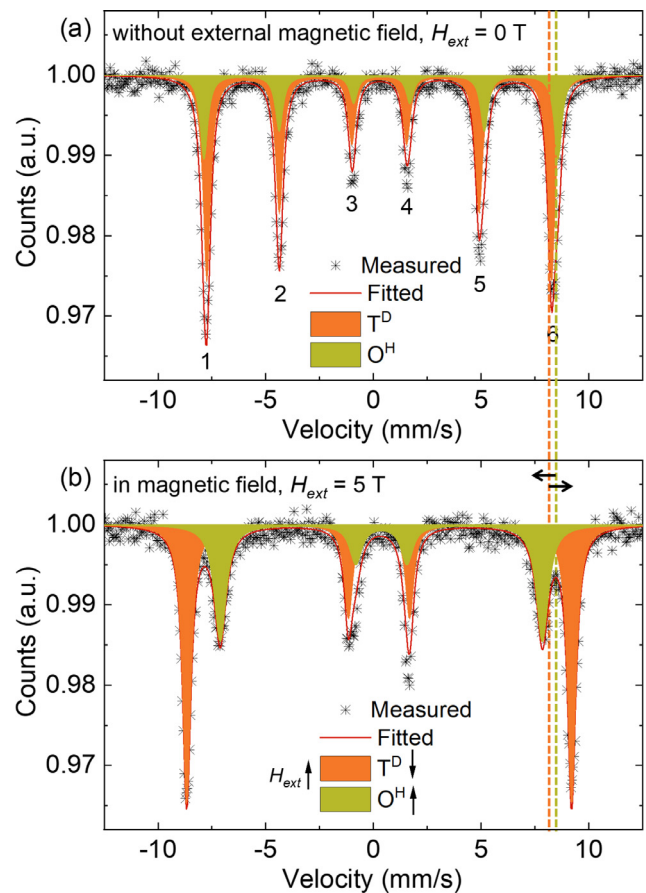
Fig. 3. Low temperature Mössbauer spectra of S-HEO (a) without magnetic field, i.e., 0 T (b) with an external magnetic field of 5 T. The orange sub-spectrum indicates the \text{Fe}^{3+} occupying the T^D sites, while the green one corresponds to the O^H sites. A clear distinction between the \text{Fe}^{3+} occupying the T^D and O^H sites can be observed in (b), while strong overlap of the features is observed in (a). The disappearance of the inner lines 2 and 5 in the (b) indicates a collinear arrangement of the Fe spins in both the sites.
