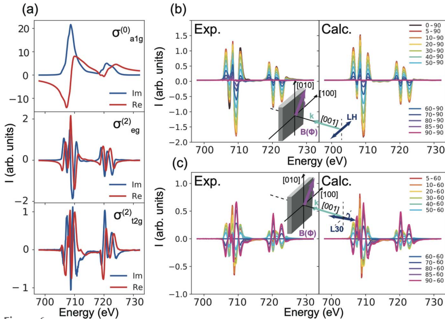
Figure 6 (a) Branching of the fundamental spectra \sigma^{(0)} and \sigma^{(2)} into \sigma_{a1g}^{(0)} , \sigma_{eg}^{(2)} and \sigma_{t2g}^{(2)} of Fe_3O_4 using a cubic expansion. (b) Fe L_{2,3} XMLD with linear horizontal polarization (labelled LH) where the XMLD signal is defined as: XMLD = XAS(\phi) - XAS(90^\circ) and \phi is the angle of the magnetic field. The measured (Exp.) and the calculated (Calc.) result from the cubic field expansion are shown in the left and right panels, respectively. (c) Fe L_{2,3} XMLD measured with linear polarization rotated 30^\circ from the [1,0,0] (labelled L30) where the XMLD signal is defined as XMLD = XAS(\phi) - XAS(60^\circ) .
