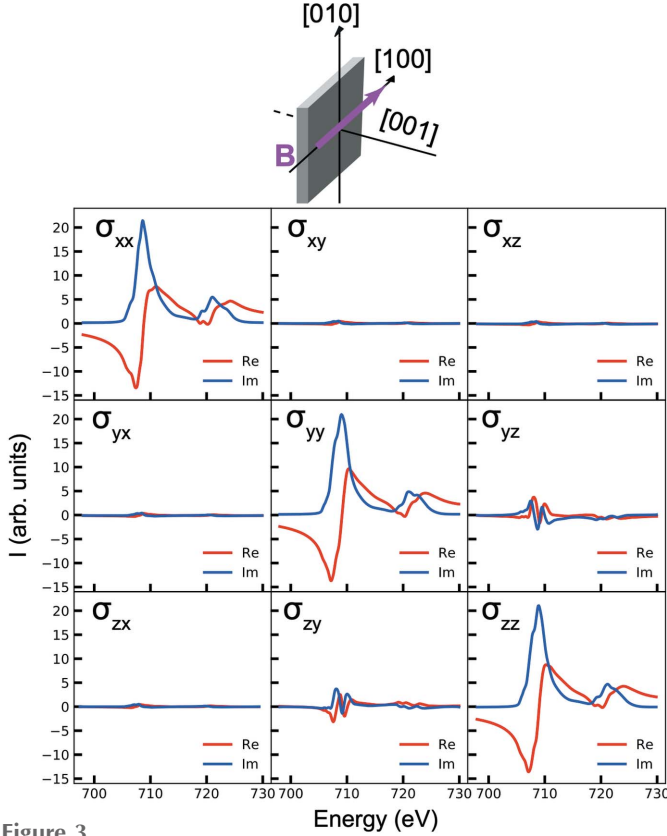
Figure 3 Fe L_{2,3} full conductivity tensor constructed for B \parallel [1,0,0] in \text{Fe}_3\text{O}_4 .
