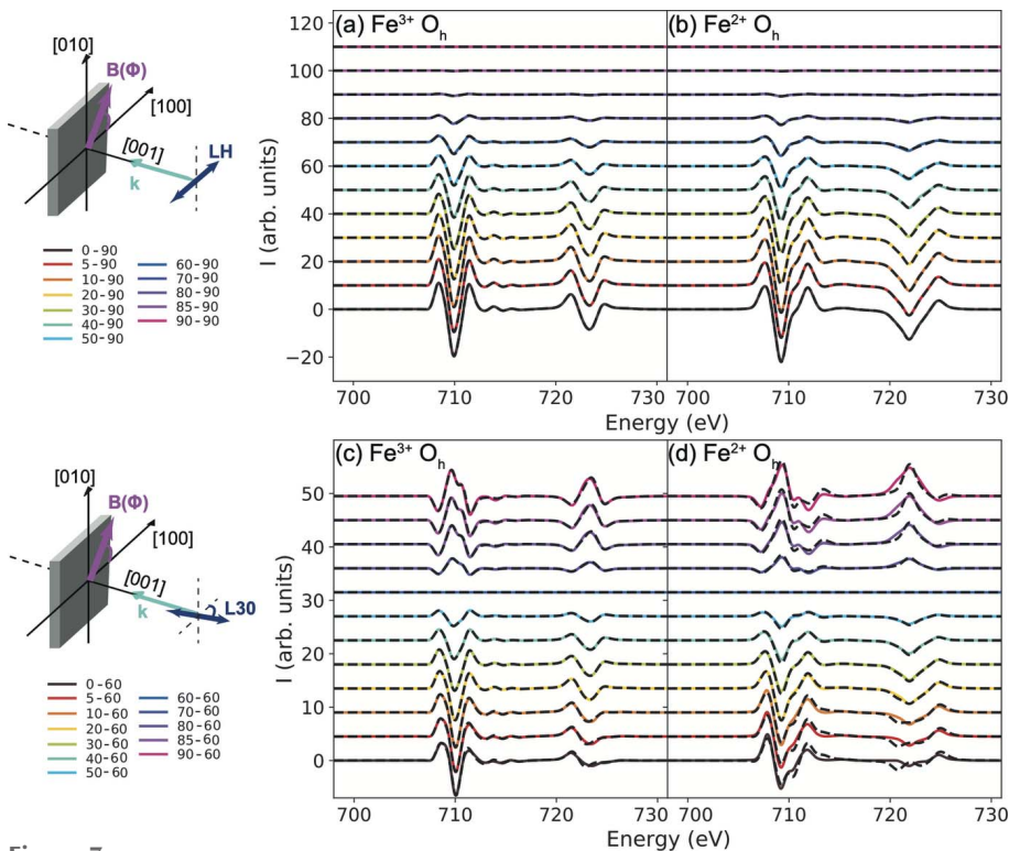
Figure 7 Computed L_{2,3} XMLD: (a) and (b) with linear polarization \parallel [1,0,0] (labelled LH) for Fe^{3+} and Fe^{2+} in O_h symmetry, respectively. The XMLD is defined as: XMLD = XAS(\phi) - XAS(90^\circ) where \phi is the angle of the magnetic field. The solid lines show XMLD computed individually for every magnetic field orientation while the dashed lines are computed using the cubic field expansion. Panels (c) and (d) are the results with linear polarization rotated 30^\circ from the [1,0,0] (labelled L30) where the XMLD is defined as: XMLD = XAS(\phi) - XAS(60^\circ) .
